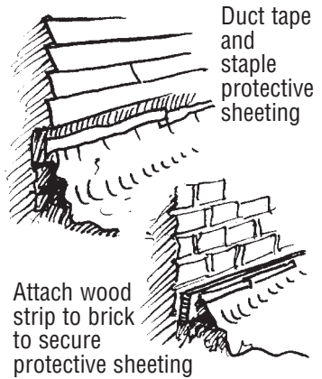
Curb edge of protective sheeting
